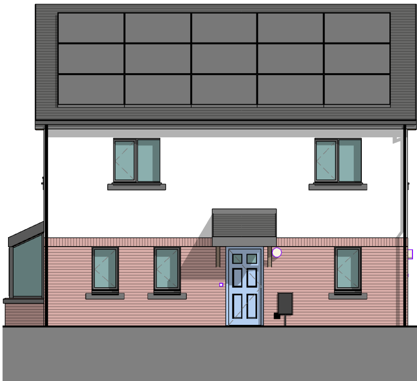
SIDE ENTRANCE ELEVATION 1 : 100
