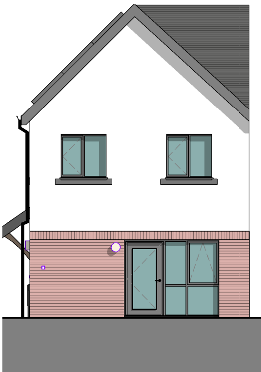
REAR GABLE ELEVATION 1 : 100
