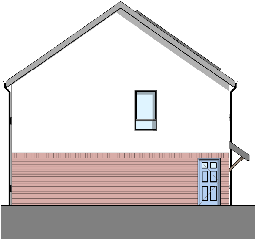
GABLE ELEVATION 1 : 100
