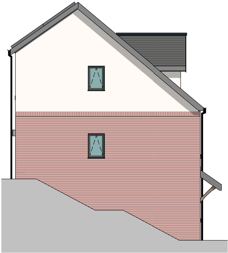
GABLE ELEVATION 1 : 100
