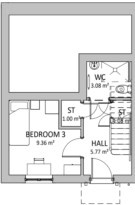
LOWER GROUND FLOOR PLAN 1 : 100
